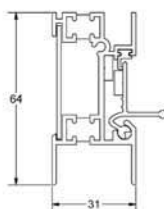
PL260P night vent assembly
