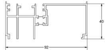
PL265 head filler
