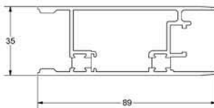
PL267 eurogroove lockstile
