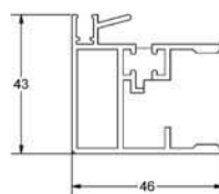
PL270 drainage tray
