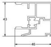
PL256 fixed interlock
