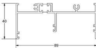
PL250 head
