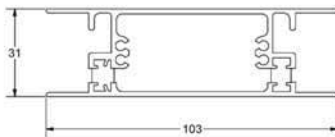
PL267 eurogroove lockstile
