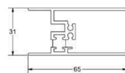
PL257 top and bottom rail
