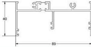
PL255 sliding interlock
