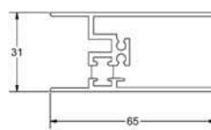
PL264 threshold
