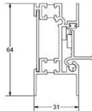
PL260P night vent assembly
