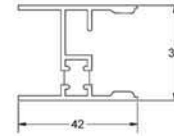
PL253 fixed stile
