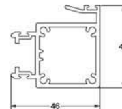
PL268 3 pane locking post
