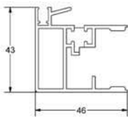
PL259 midrail
