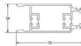
PL269 4 pane meeting stile
