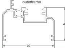
RD03 deep direct fix outerframe
