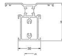
IG204 28mm bead (IG203/IG205)
