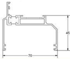
TW142 externally glazed euro vent
