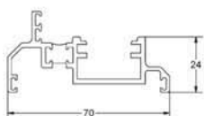
RD02 slim direct fix outerframe
