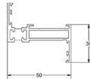
TW102 odd leg outerframe/ cockspur vent
