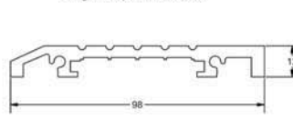
RD200SR single ramp low threshold
