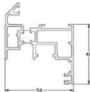
TW115 wide midrail
