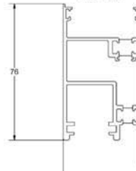
RD09 slave stile
