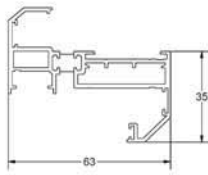
TW105 20mm mullion/transom
