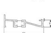
RD04 timber fix drainage tray
