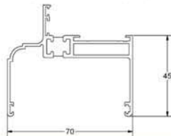
TW143 externally glazed ovolo vent
