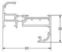
TW143 externally glazed ovolo vent
