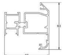
IG205 internally glazed ovolo vent
