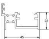
RD01 timber fix outerframe
