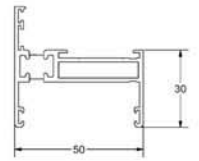
IG205 internally glazed ovolo vent
