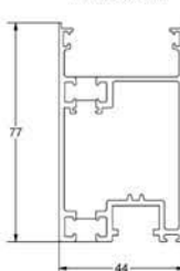
RD07 lock/hinge stile
