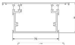
TW116 4/6mm single glazing
