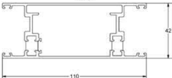
RD10 midrail
