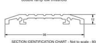
RD200DR double ramp low threshold
